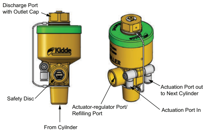
Figure 4. Valve Components
