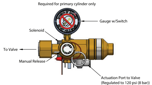
Figure 5. Release Unit
