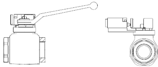
Figure 14. Lockout Valve
